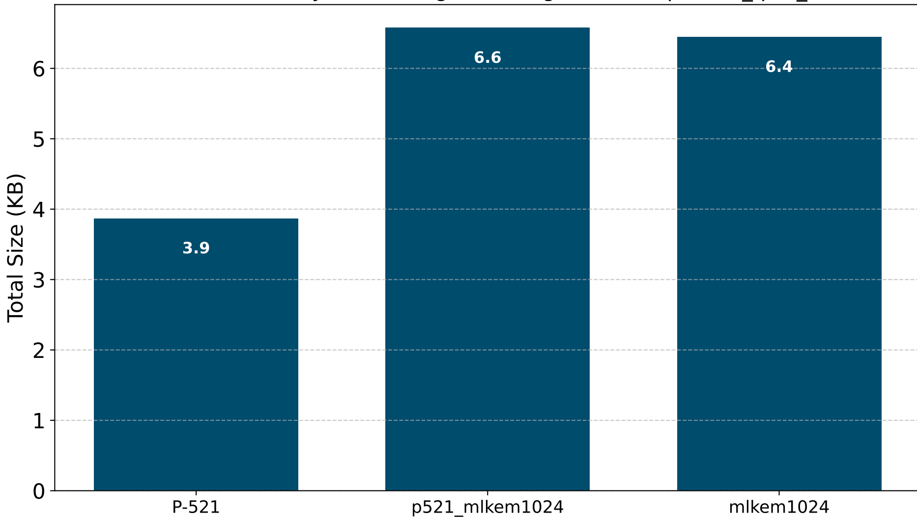
Total traffic size by KEM for signature algorithm secp521r1_quic_size
